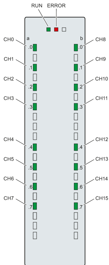
图 5-1 LED 模块的指示灯DI 16x230VAC BA
